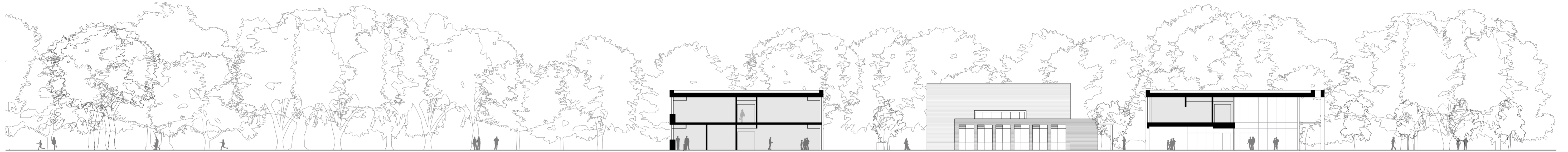
Cross Section Through Entrance And Classroom Block
