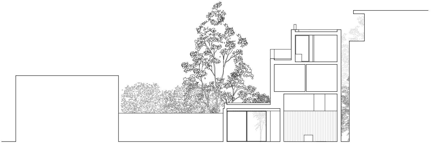
Section CC
