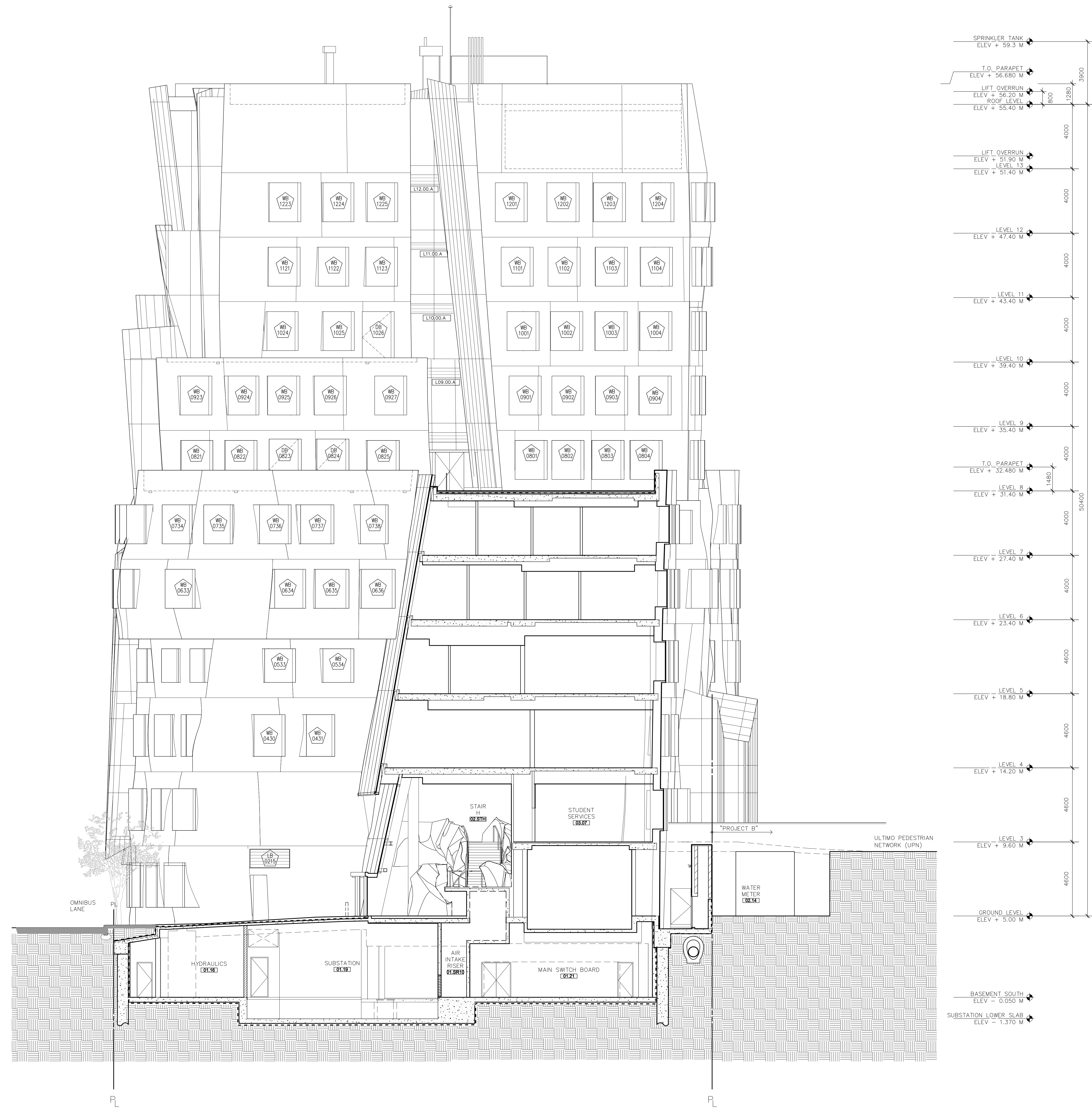
BUILDING SECTION SOUTH VIEW
