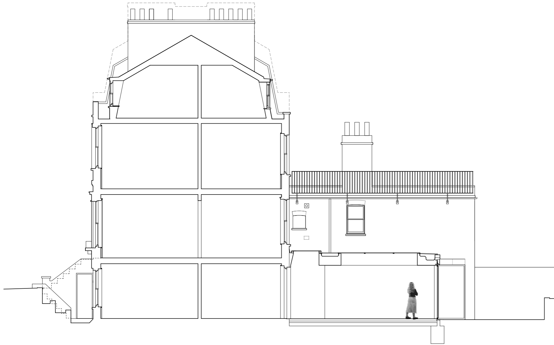
Proposed Long Section A-A
