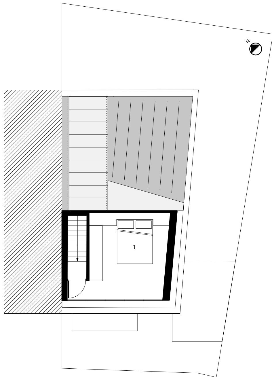
THIRD FLOOR PLAN MILSON ROAD HOUSE
