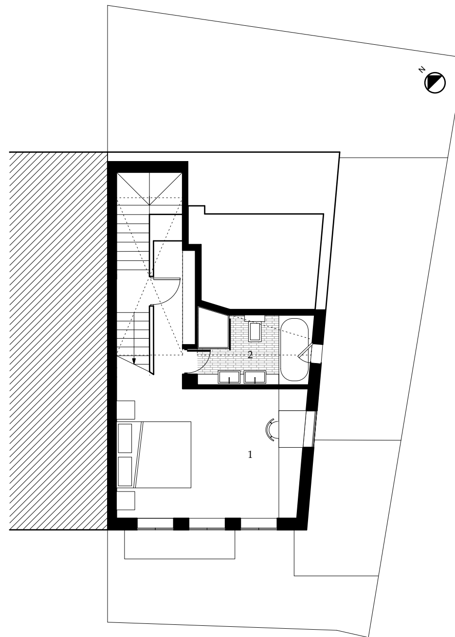
SECOND FLOOR PLAN MILSON ROAD HOUSE
