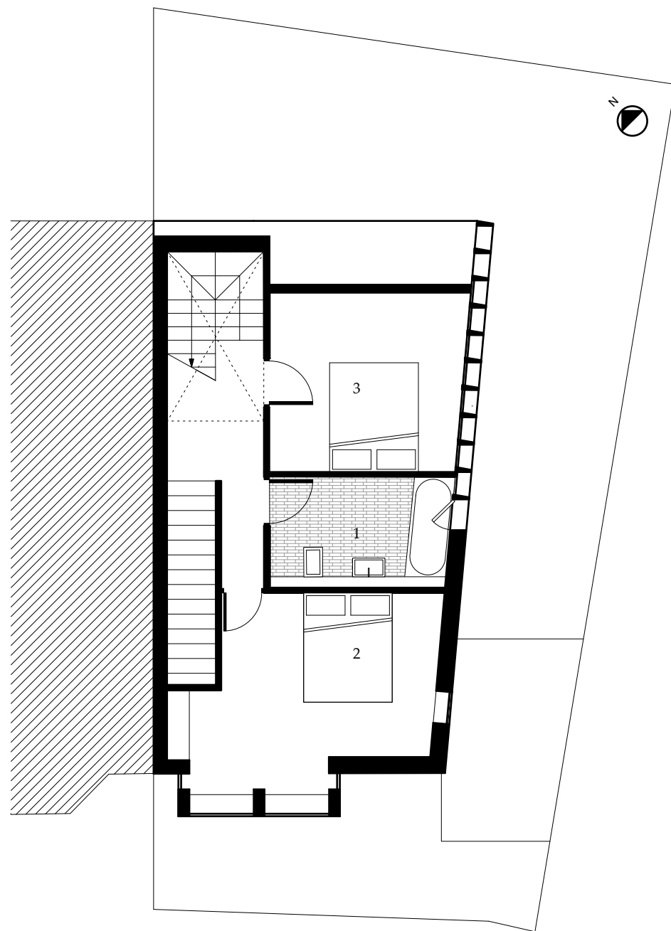
FIRST FLOOR PLAN MILSON ROAD HOUSE
