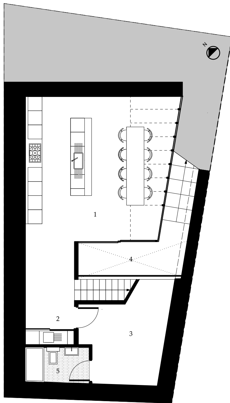
BASEMENT PLAN MILSON ROAD HOUSE
