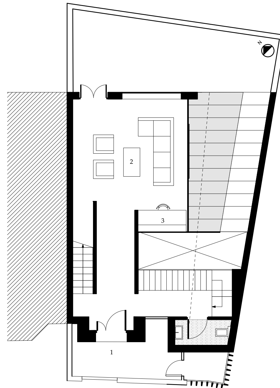
GROUND FLOOR PLAN MILSON ROAD HOUSE
