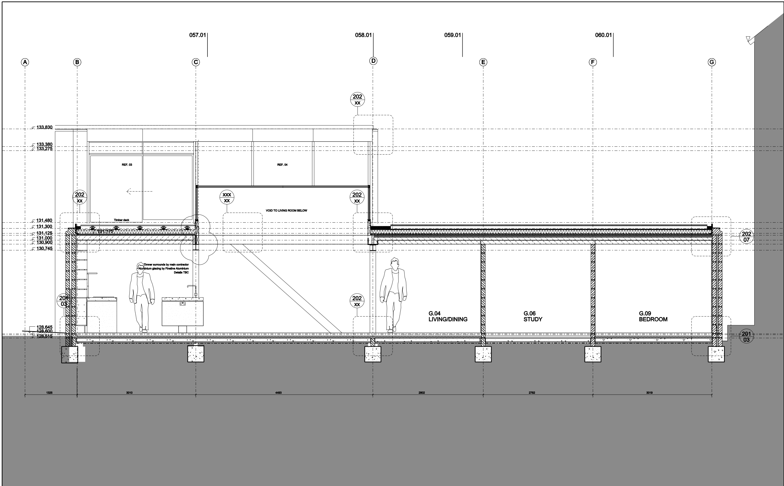
01 Proposed Section B-B
