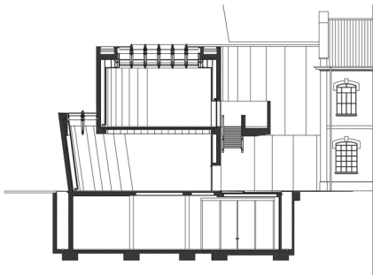
cross section through galleries
