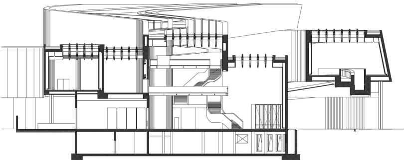
cross section through galleries and main lobby
