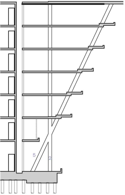
Section: east facade
