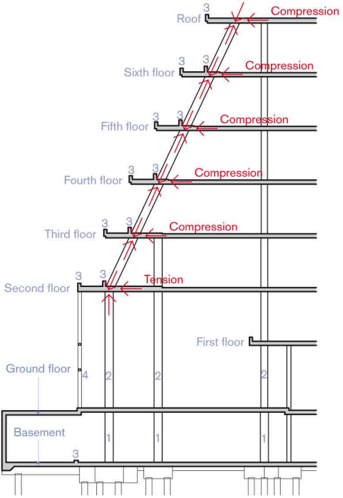
Section: west facade
