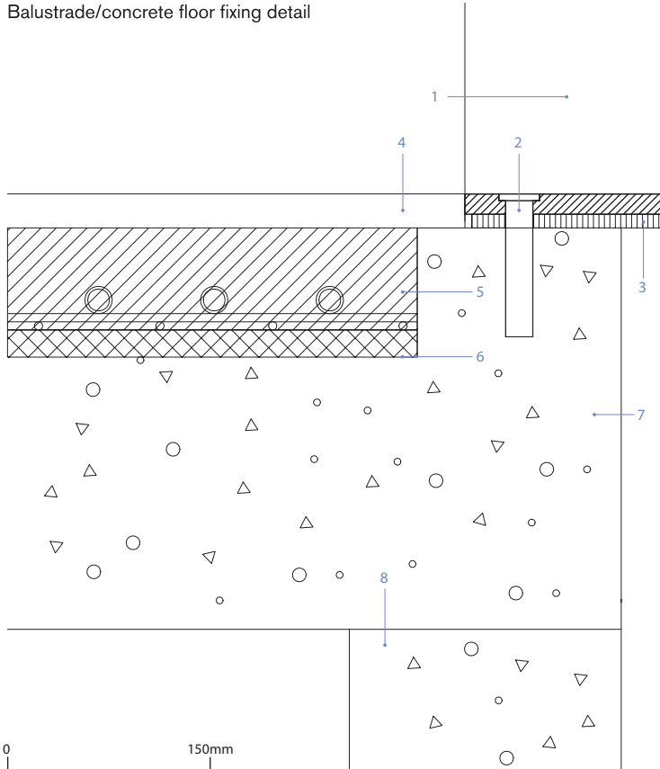
Balustrade/concrete floor fixing detail
