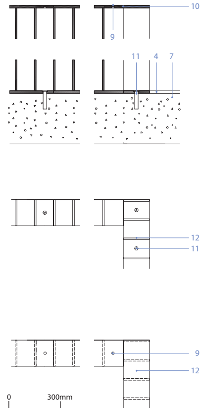
Balustrade fixing detail
